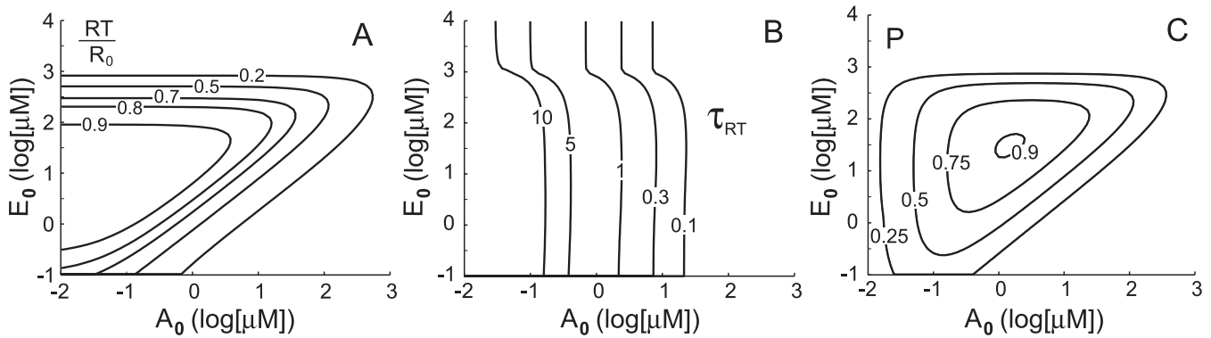
Figure 4. The GTPase Activity and the Overall Cycling Performance Are Improved by the Introduction of a GEF-Activating GTPase Effector S. The profiles of the GTPase activity (A), recovery time (B), and performance index (C) are plotted as contour lines. Note the increase in the area of the optimal control and its shift toward lower GEF concentrations in comparison with Figure 3C. doi:10.1371/journal.pcbi.0020172.g004
