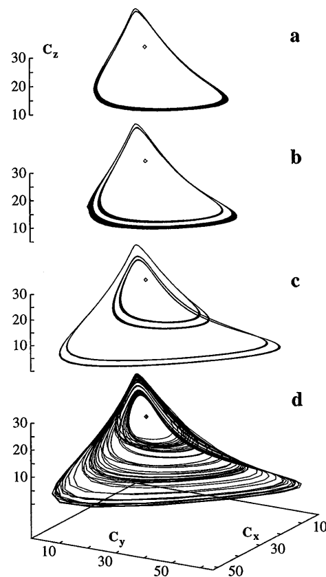
FIG. 2. Phase space trajectories \mathbf{c}(r, \theta, t) for \kappa_2 = 1.567 and the other rate parameters as in Fig. 1 at fixed \theta = (3/4)\pi for three values of r : (a) period-1 limit cycle at r = 0.194 ; (b) period-2 orbit at r = 0.206 , and (c) period-4 orbit at r = 0.344 . The scaled diffusion coefficient is D\Delta t/(\Delta x)^2 = 0.01 and no-flux boundary conditions are used. (d) Local chaotic dynamics at a point in Fig. 1 far removed from a defect.
