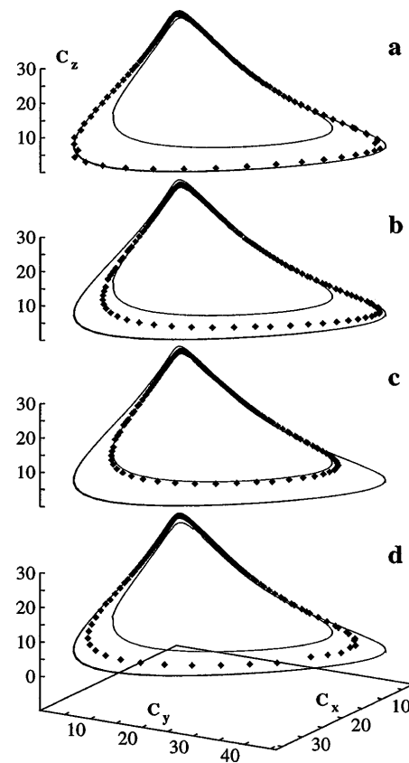
FIG. 3. Plots of S in the \mathbf{c} phase space for r = 0.219 for four different times t_i : (a) t_1 = 0.0 ; (b) t_2 = 0.209 ; (c) t_3 = 0.326 ; and (d) t_4 = 0.721 . Time is expressed in the fractions of average time period of P-2. S is shown as filled diamonds while the solid curve represents one period of the P-2 orbit at [r = 0.219, \theta = (3/4)\pi] . The simulation conditions are the same as in Fig. 2.
